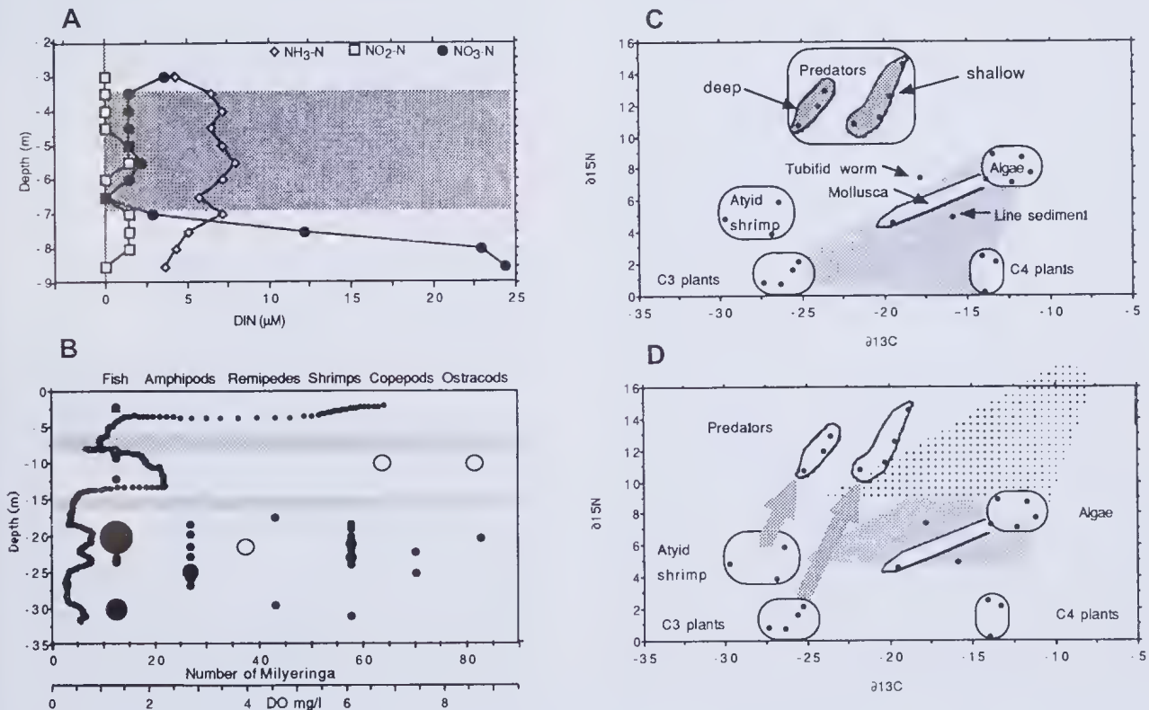
Figure 3. A; Vertical profile with depth of the dissolved inorganic nitrogen species (DIN \mu\text{M} ) \text{N-NH}_3 , \text{N-NO}_2 , \text{N-NO}_3 , shading denotes the region of elevated \text{H}_2\text{S} concentration (see Fig 2F). B; vertical distribution of sightings of the fauna in Bundera Sinkhole reported by divers, a) the closed circles denote the vertical distribution of the taxon named at the head of the column, b) the open circles denote the number of blind gudgeons ( Milyeringa veritas ) counted at one occasion at each of three depths (second bottom scale), c) the curve denotes the DO concentration (bottom scale), d) the grey bands denote the zones of elevated hydrogen sulphide concentration (see figure 9). These data are illustrative only as no regular sampling has been conducted through time. C; scatter plot of ^{15}\text{N} ‰ and ^{13}\text{C} ‰ values for samples from Bundera Sinkhole. If the food source is hypothesised to be some mix of \text{C}_3 and \text{C}_4 plants and algae then the average ^{13}\text{C} and ^{15}\text{N} values would lie in the polygon linking these data (shaded area). Data for plants with \text{C}_3 and \text{C}_4 metabolism, and algae are outlined, as are predators (left group, deep cave Milyeringa ; right group, shallow cave Milyeringa [x3], gerrid [x1]), molluscs and worms. D; scatter plot of ^{13}\text{C} ‰ and ^{15}\text{N} ‰ values for samples from Bundera Sinkhole. If the food source is hypothesised to be some mix of \text{C}_3 and \text{C}_4 plants and algae then the average ^{13}\text{C} and ^{15}\text{N} values would lie in the polygon linking these data. This is represented as a shaded area but it has been displaced by one (heavy shading) and two (light shading) trophic increments of respectively 2 ‰ for ^{13}\text{C} and 4 ‰ for ^{15}\text{N} .
